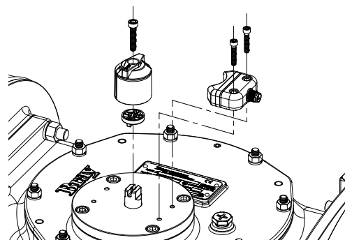
Series 98 Actuator
