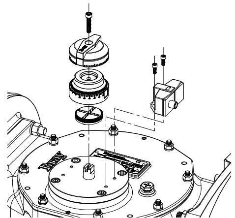
Series 98 Actuator
