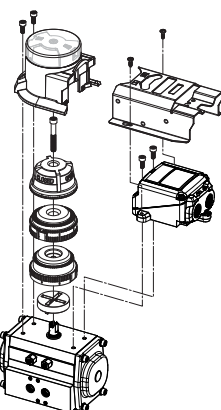
Series 92/93 Actuator
