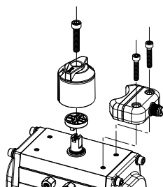
Series 92/93 Actuator
