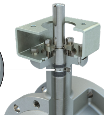
Solid Seal Ring
