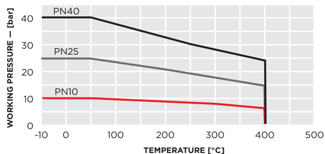
MAXIMUM WORKING PRESSURE VS TEMPERATURE 1
