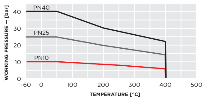
MAXIMUM WORKING PRESSURE VS TEMPERATURE 1
