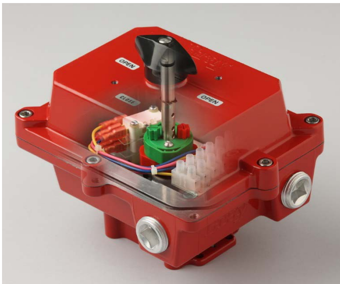
Figure 2. Series 50 cutaway showing the cams and switches.
