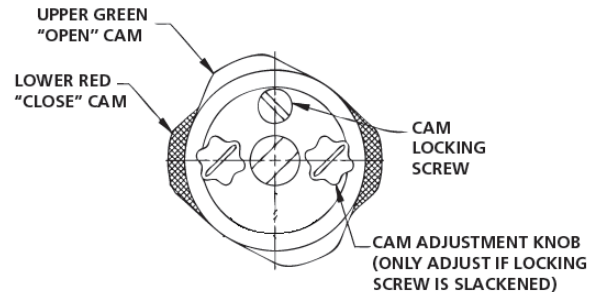
Figure 3. Top view of the cam shaft assembly.
