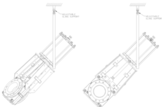
Figura 5: Valve with Actuator at 45°
