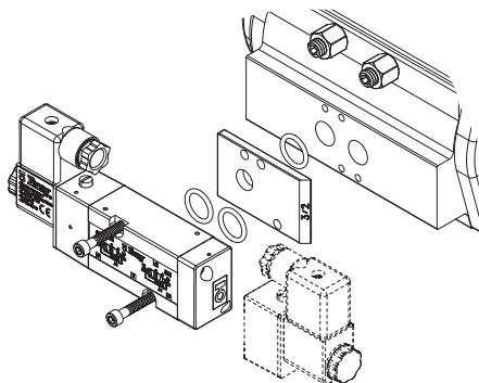
Figure 4: 3/2 Installation
