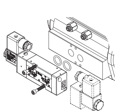
Figure 3: 5/2 Installation
