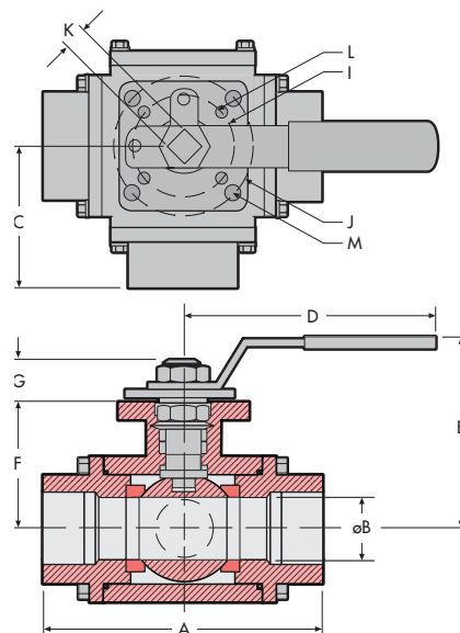
MPT/MPS/MPB - 230* - 1/4" - 2" shown
