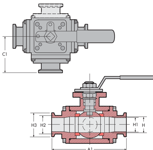
MPC230 - 1/2" - 2" shown
