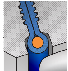
Seat non-compressed as disc approaches.
