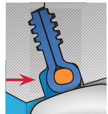
Disc in closed position; line pressure applied from the left.
